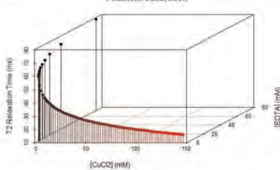
Figure 1. Combined logarithmic relation among [\text{EDTA}] , [\text{CuCl}_2] concentrations and T2 relaxation time. Density was not included in this three-dimensional plot since it depends mostly on [\text{CuCl}_2] only.
