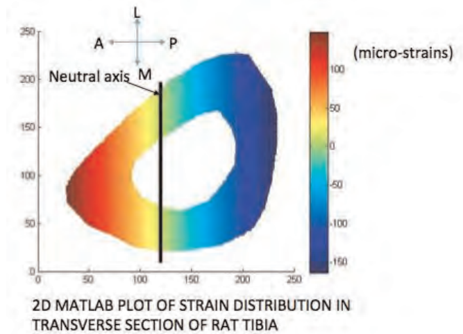
Fig 2-2D Matlab Plot of Strain Distribution in transverse section of rat left tibia
