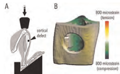
Figure 1. (A) Tibial cortical defect subjected to axial loading. (B) Estimated longitudinal strain.
